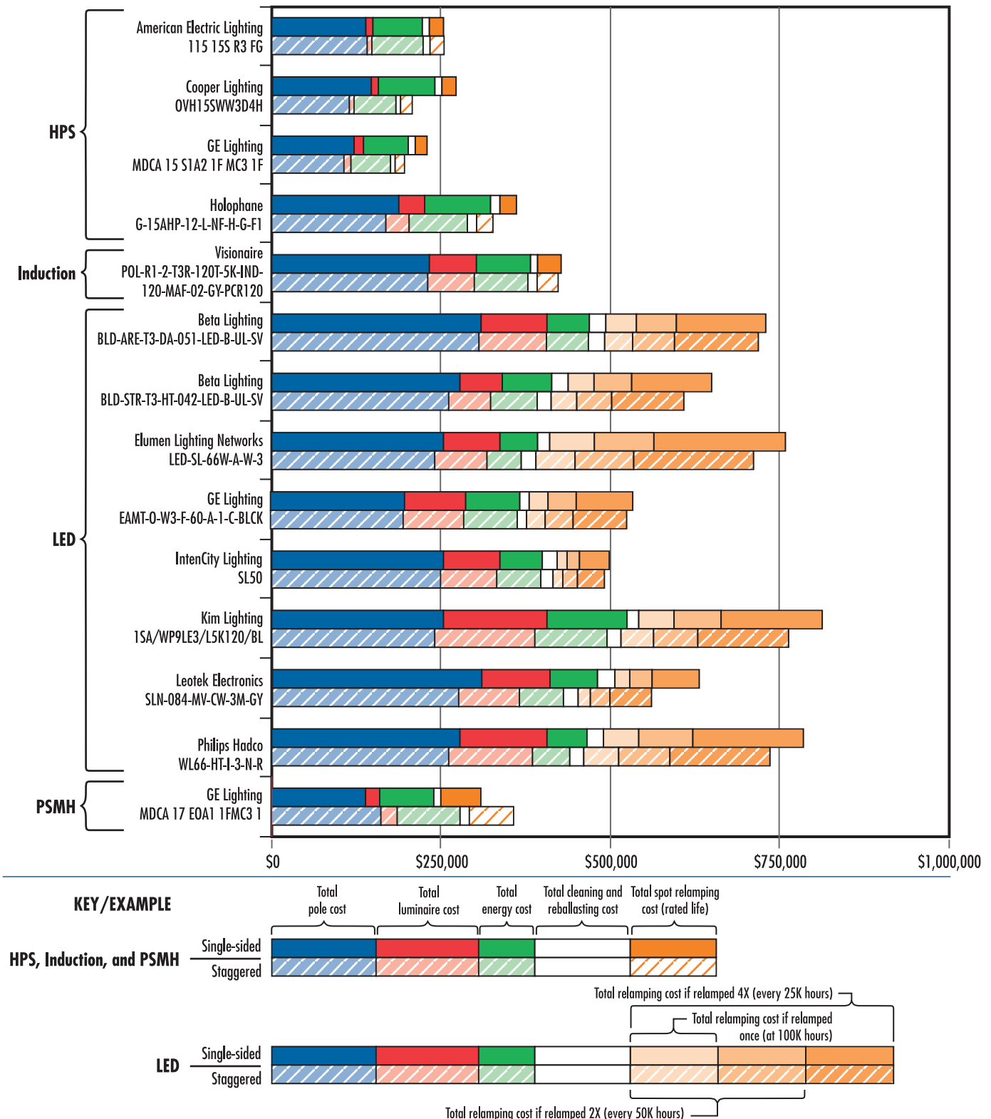
Figure 8. Life Cycle Cost per Mile over 27 Years
