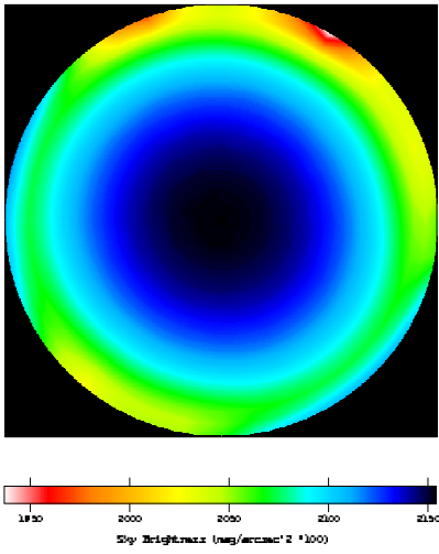
Figure 10. Night sky brightness in V band at Mt. Graham Observatory, USA in polar coordinates for atmospheric clarity K' = 0.5 . The figure is plotted with East at bottom, North at left.
